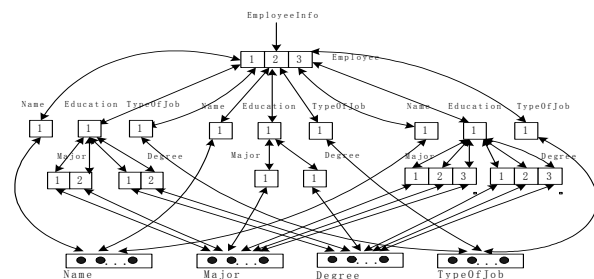
Figure 2. IX-tree of EmployeeInfo.xml
