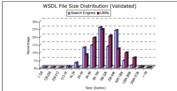
Figure 7. WSDL file size distribution (validation)
