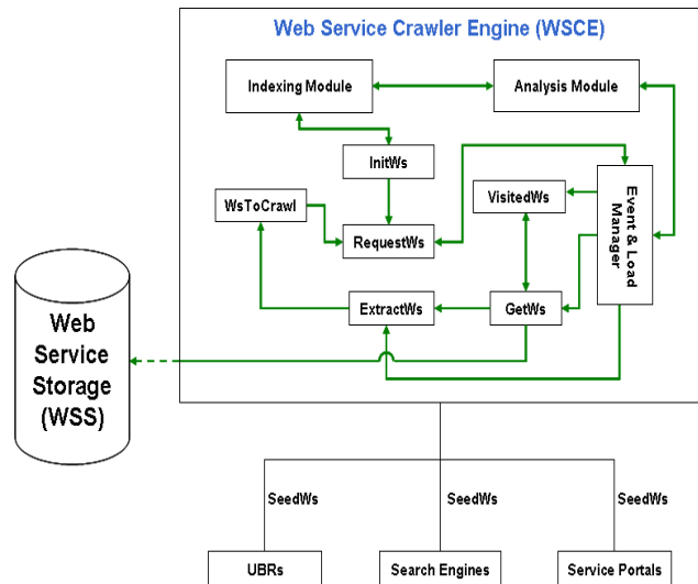
Figure 1. Web Service Crawler Engine (WSCE)
