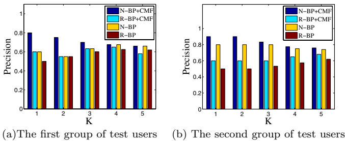
Figure 6: Precision at varying K .
