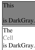
Figure 9: Counter-example layouts
