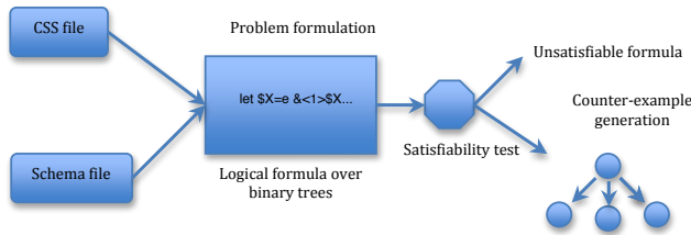
Figure 7: Overall architecture
