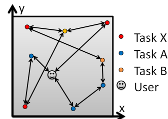
Figure 4: Network Model
