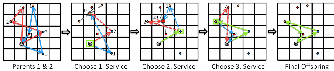
Figure 15: Localizer Crossover
