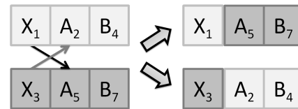
Figure 14: Single-Point Crossover
