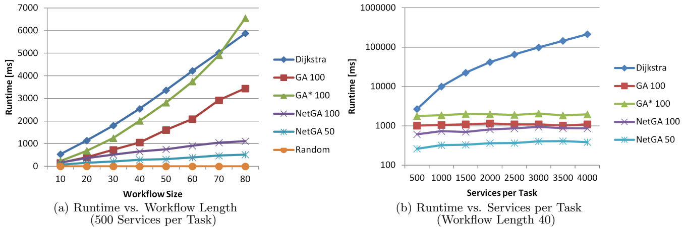
Figure 19: Runtime vs. Increasing Problem Size
