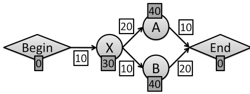
Figure 8: QoS of a Workflow
