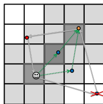
Figure 13: Localizer Mutation
