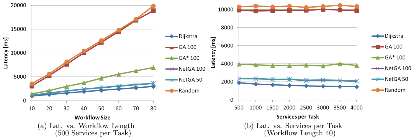
Figure 17: Latency vs Increasing Problem Size
